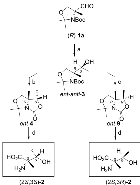
Scheme 4. Reagents and conditions: (a) MeMgBr, THF, -78^\circ\text{C} , 4 h, 87%; (b) NaH, DMF, 25^\circ\text{C} , 6 h, 88%; (c) \text{TiF}_2\text{O} , 2,6-di- tert -butyl-4-methylpyridine, \text{CH}_2\text{Cl}_2 , 0^\circ\text{C} , 5 min, 88%; (d) (i) 4 M HCl/THF (1:1), 25^\circ\text{C} , 2 h; (ii) Jones reagent, acetone, 3 h, 0^\circ\text{C} and another 3 h, 25^\circ\text{C} ; (iii) 6 M HCl reflux, 48 h; (iv) propylene oxide/EtOH (1:3), reflux, 48 h (52% from ent-4 or ent-9 ).
